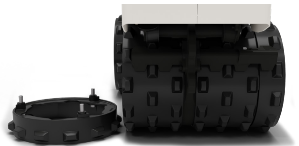
REMOVABLE EXTENSIONS
